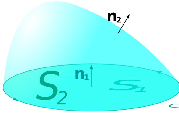
Figure 6: Stokes' Theorem can be used for any surface S whose boundary is the curve C .
