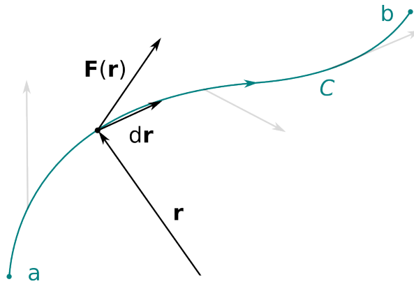
Figure 1: The work from a varying force is found by chopping the trajectory \mathcal{C} into tiny segments and summing up the contributions from each segment.
